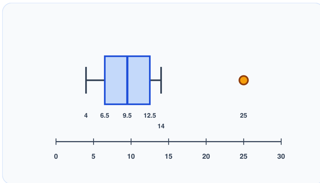
Modified Boxplot for the Data
