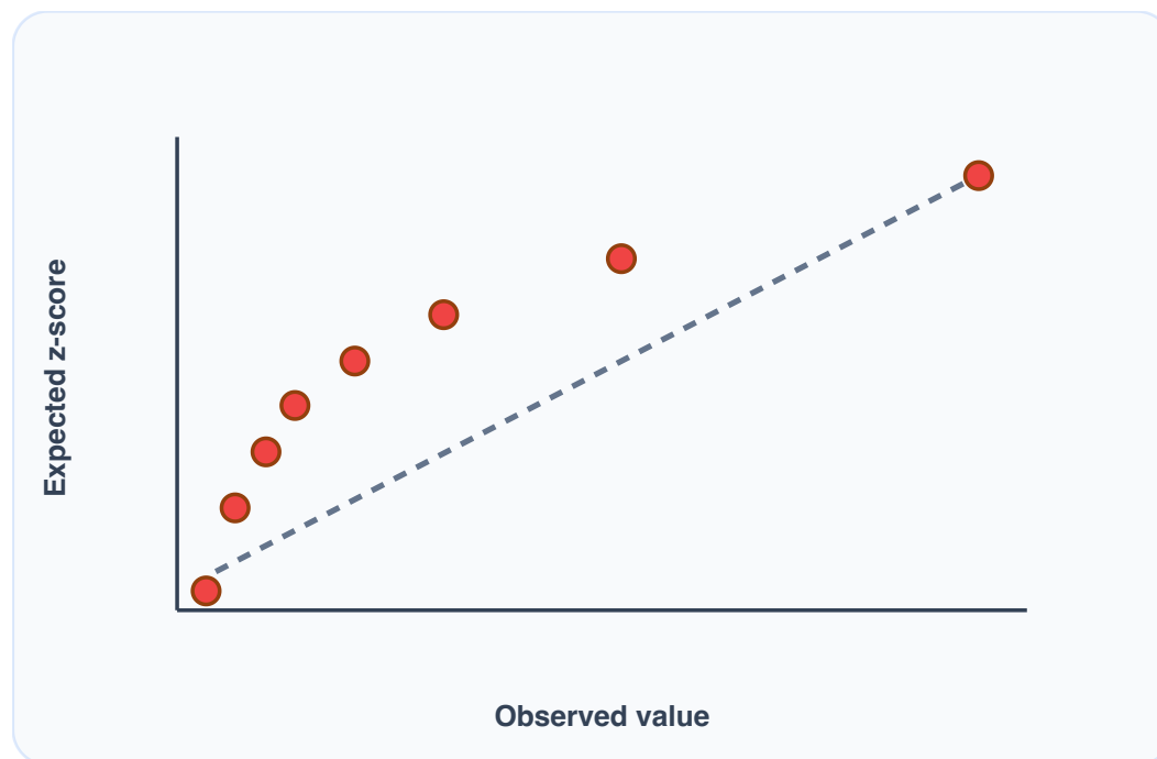
Curved Normal Probability Plot
