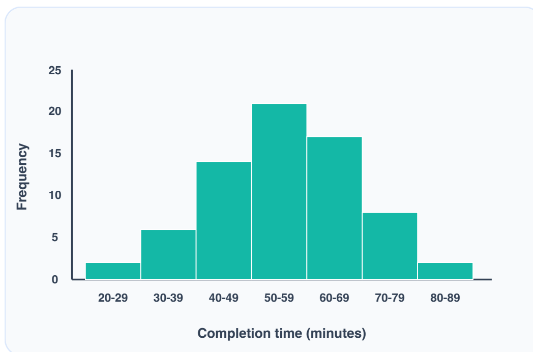
Workshop Completion Times
