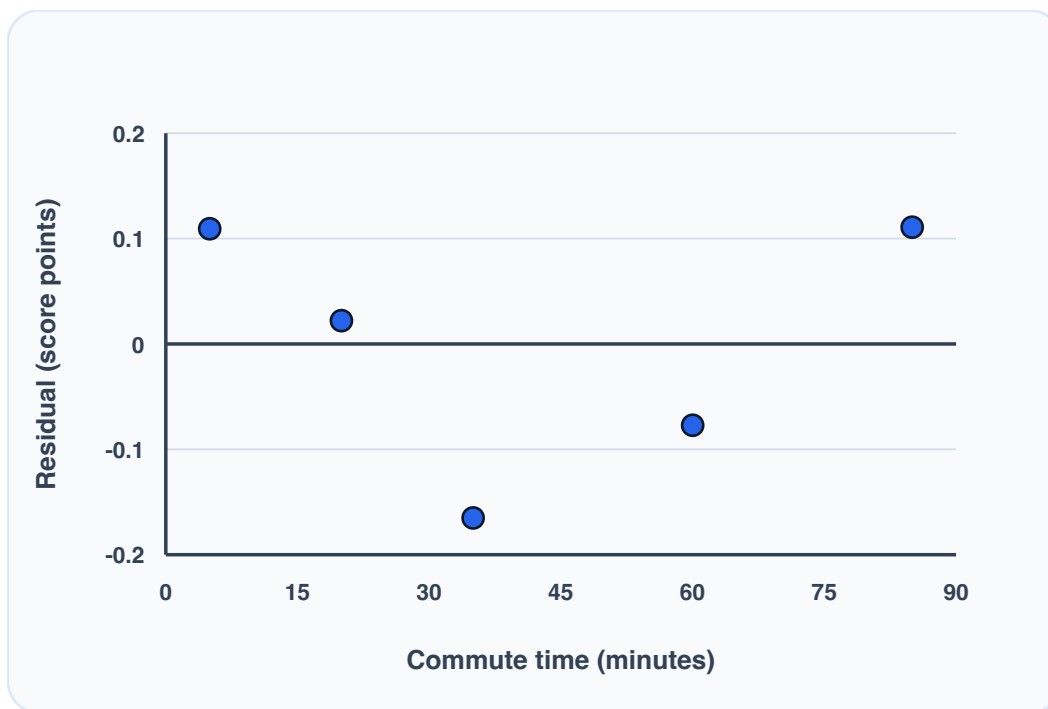
Commute Time and Well-Being: Residual Plot
