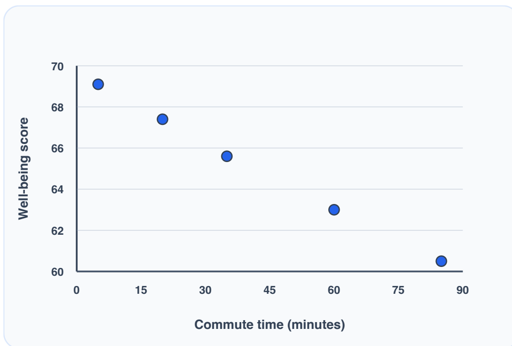
Commute Time and Well-Being
